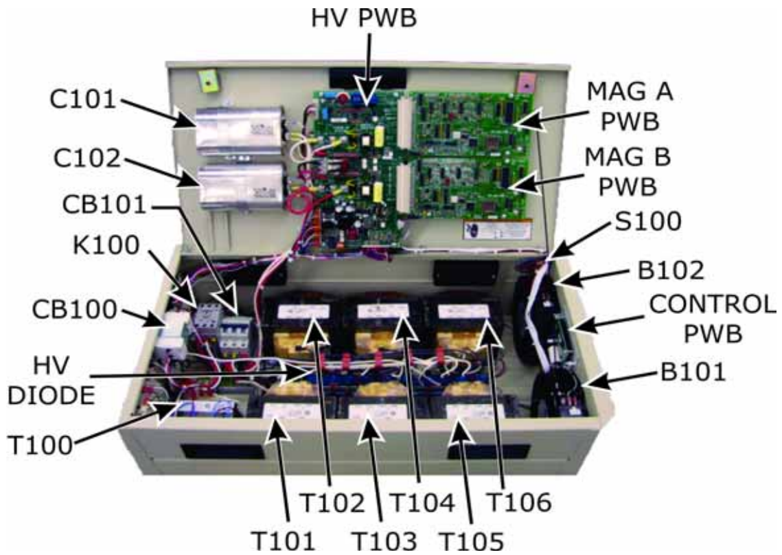
VPS Power Supply Components
