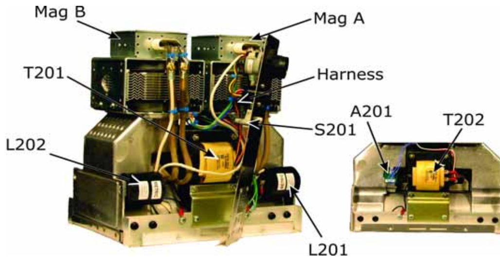
I250 Irradiator Components
