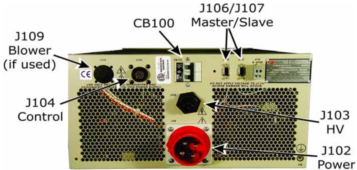
VPS Power Supply Components (Rear)
