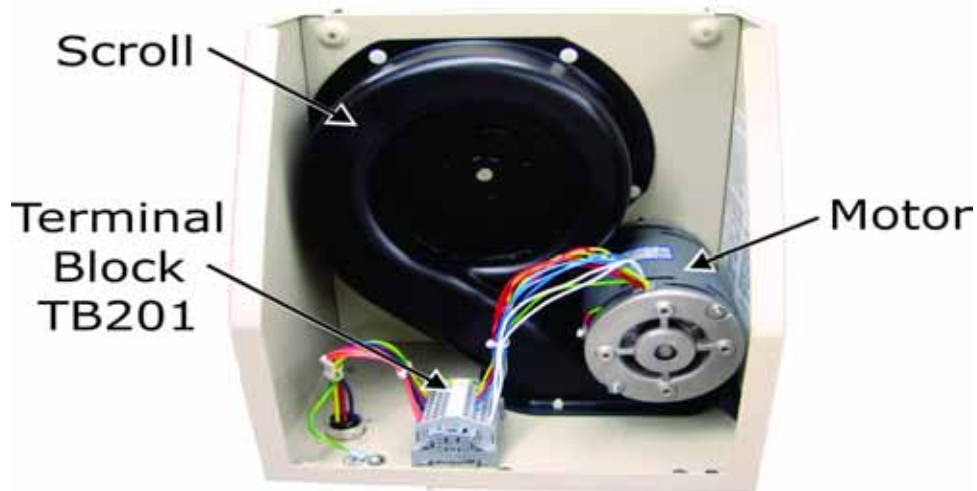
K250 Irradiator Components
